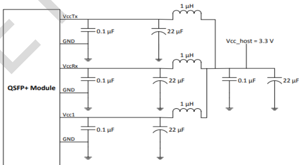
FIGURE 5-4 RECOMMENDED HOST BOARD POWER SUPPLY FILTERING
